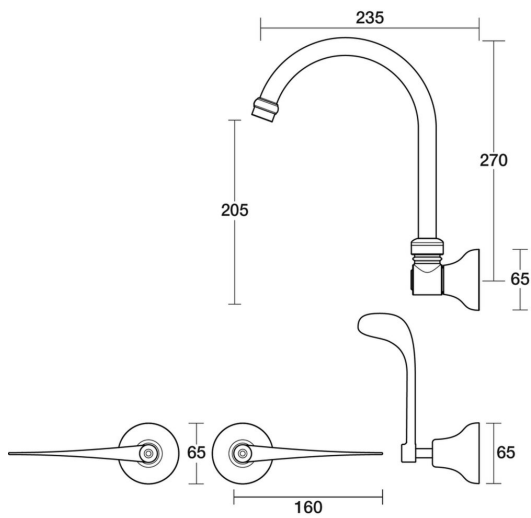
Bell Sink Set Wall Swivel DDA Compliant Extended Lever Ceramic Disc B32.052.5.01 - Chrome
