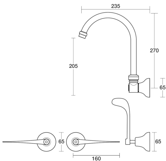
Bell Sink Set Wall Swivel DDA Compliant Extended Lever Ceramic Disc B32.052.5.13 - Gold / White
