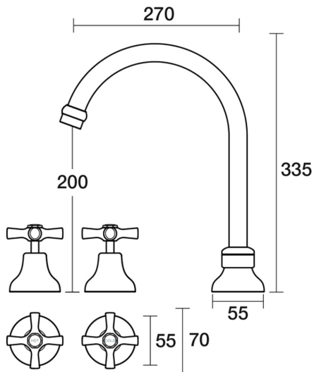
Bell Sink Set XL Hob Swivel B32.053.1.03 - Chrome / White
