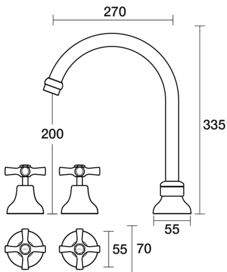
Bell Sink Set XL Hob Swivel B32.053.1.05 - Chrome / Apricot
