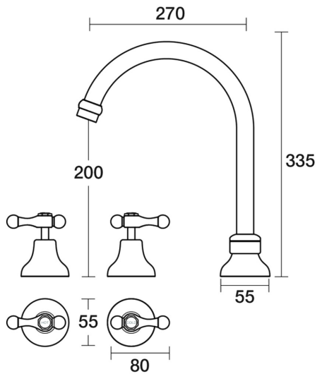
Bell Sink Set XL Hob Swivel Lever Ceramic Disc B32.053.3.03 - Chrome / White
