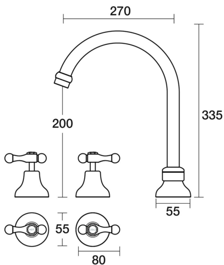
Bell Sink Set XL Hob Swivel Lever Ceramic Disc B32.053.3.10 - Chrome / Gold
