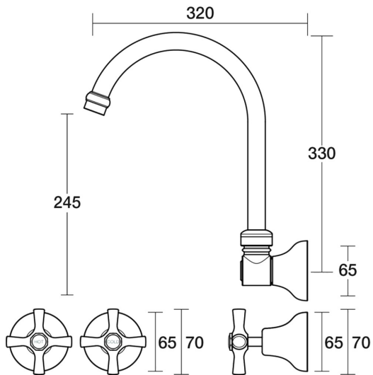
Bell Sink Set XL Wall Swivel B32.054.1.16 - Gold / Sienna Red
