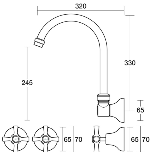
Bell Sink Set XL Wall Swivel B32.054.1.19 - 23k Brushed Brass Gold
