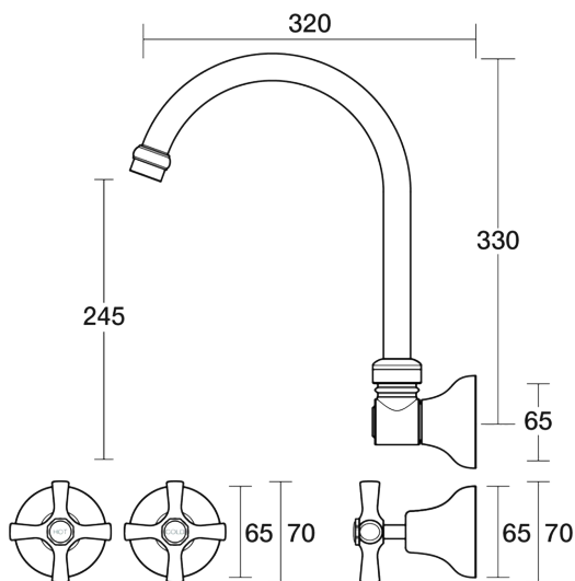
Bell Sink Set XL Wall Swivel Ceramic Disc B32.054.2.01 - Chrome
