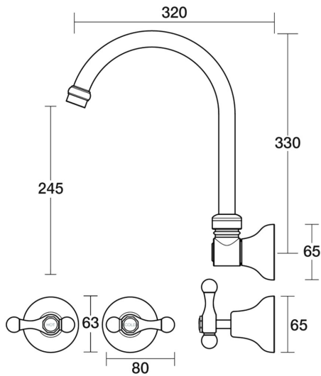
Bell Sink Set XL Wall Swivel Lever Ceramic Disc B32.054.3.04 - Chrome / Ivory
