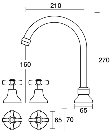
Bell Spa Set Hob Swivel Ceramic Disc
