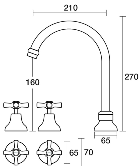
Bell Spa Set Hob Swivel Ceramic Disc B32.061.2.11 - 23k Gold
