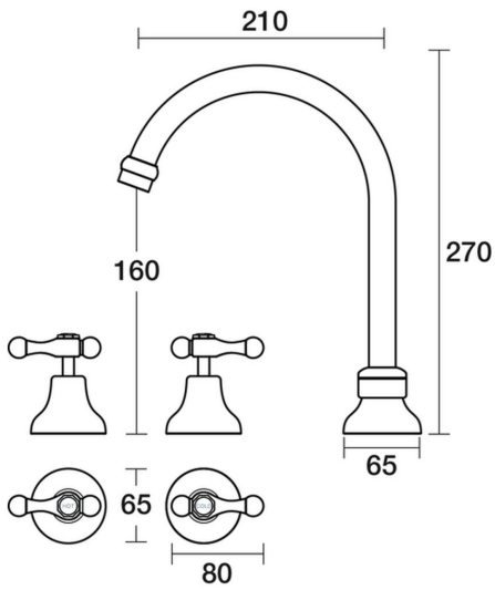
Bell Spa Set Hob Swivel Lever Ceramic Disc B32.061.3.01 - Chrome
