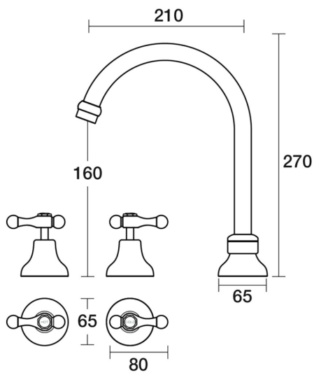
Bell Spa Set Hob Swivel Lever Ceramic Disc B32.061.3.03 - Chrome / White
