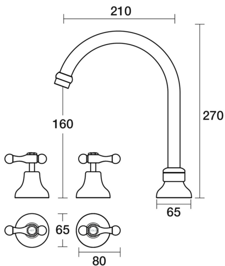
Bell Spa Set Hob Swivel Lever Ceramic Disc B32.061.3.05 - Chrome / Apricot
