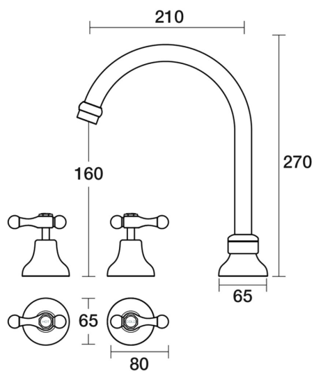
Bell Spa Set Hob Swivel Lever Ceramic Disc B32.061.3.10 - Chrome / Gold
