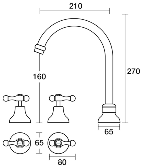
Bell Spa Set Hob Swivel Lever Ceramic Disc B32.061.3.14 - Gold / Ivory
