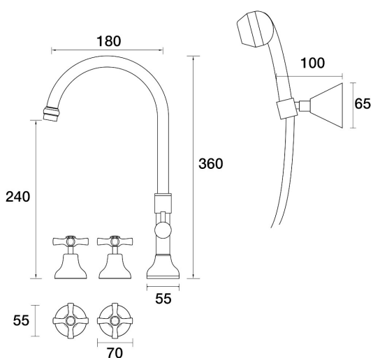
Bell Spa Set Hob Swivel Divertor Set with Handshower & Bracket B32.061.4.12 - 23k Brushed Gold
