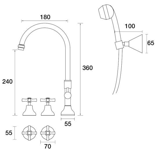
Bell Spa Set Hob Swivel Divertor Set with Handshower & Bracket B32.061.4.16 - Gold / Sienna Red
