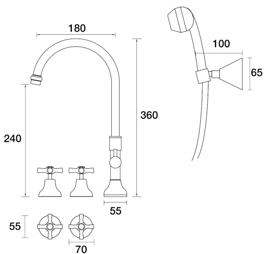
Bell Spa Set Hob Swivel Divertor Set with Handshower & Bracket Ceramic Disc B32.061.5.15 - Gold / Apricot
