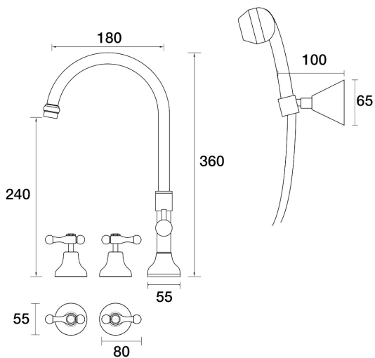
Bell Spa Set Hob Swivel Divertor Set with Handshower & Bracket Lever Ceramic Disc B32.061.6.04 - Chrome / Ivory
