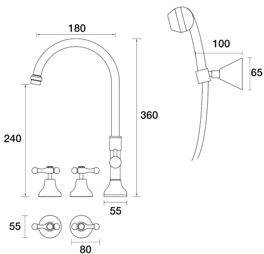
Bell Spa Set Hob Swivel Divertor Set with Handshower & Bracket Lever Ceramic Disc B32.061.6.19 - 23k Brushed Brass Gold
