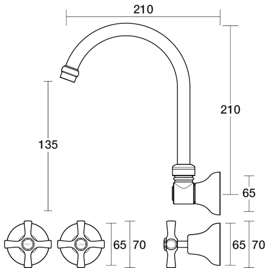
Bell Spa Set Wall Swivel B32.062.1.01 - Chrome
