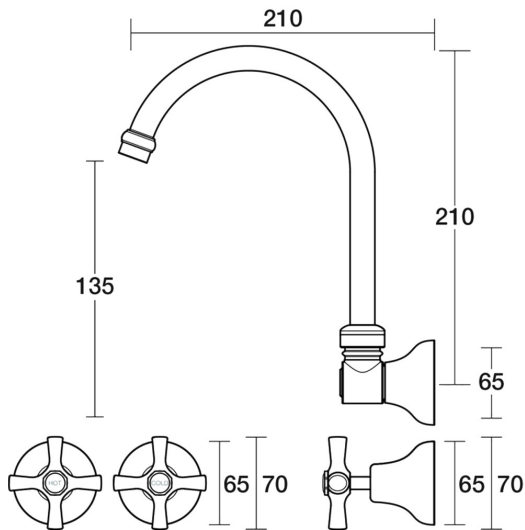
Bell Spa Set Wall Swivel B32.062.1.15 - Gold / Apricot
