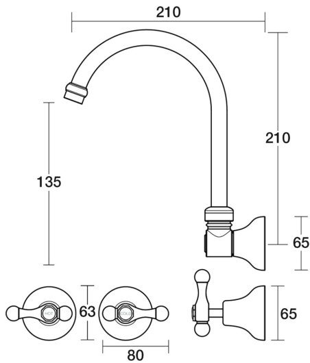
Bell Spa Set Wall Swivel Lever Ceramic Disc B32.062.3.03 - Chrome / White
