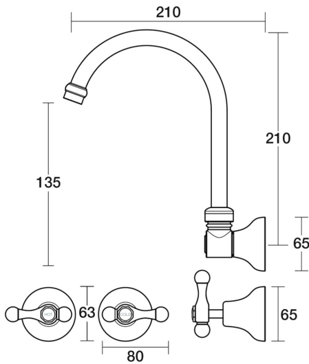
Bell Spa Set Wall Swivel Lever Ceramic Disc B32.062.3.13 - Gold / White
