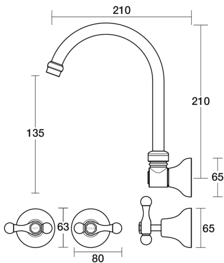
Bell Spa Set Wall Swivel Lever Ceramic Disc B32.062.3.14 - Gold / Ivory
