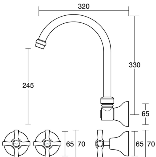
Bell Spa Set XL Wall Swivel B32.064.1.05 - Chrome / Apricot
