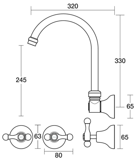
Bell Spa Set XL Wall Swivel Lever Ceramic Disc B32.064.3.15 - Gold / Apricot
