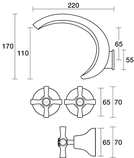
Bell Spa Set Wall Deluxe B32.066.1.03 - Chrome / White
