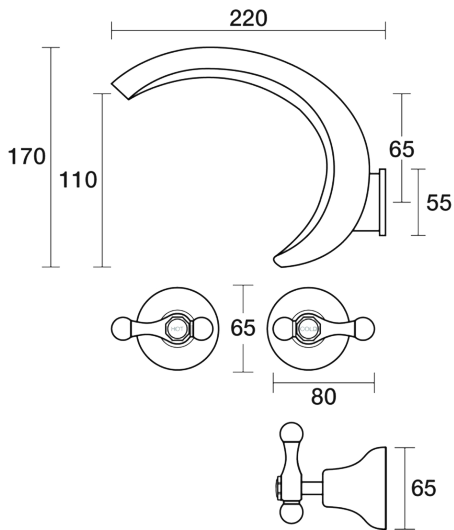
Bell Spa Set Wall Deluxe Lever Ceramic Disc B32.066.3.01 - Chrome
