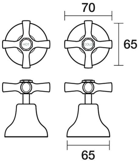
Bell Top Assemblies Wall Pair Ceramic Disc B32.082.2.04 - Chrome / Ivory
