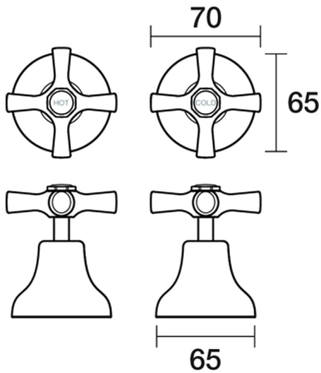
Bell Top Assemblies Wall Pair Ceramic Disc B32.082.2.06 - Chrome / Sienna Red
