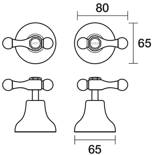
Bell Top Assemblies Wall Pair Lever Ceramic Disc B32.082.3.01 - Chrome
