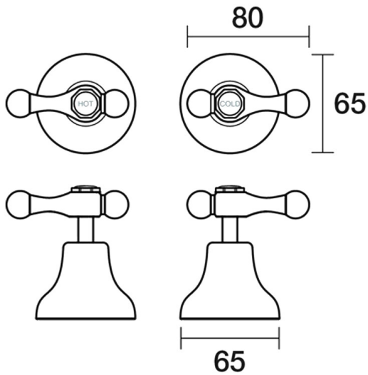
Bell Top Assemblies Wall Pair Lever Ceramic Disc B32.082.3.06 - Chrome / Sienna Red
