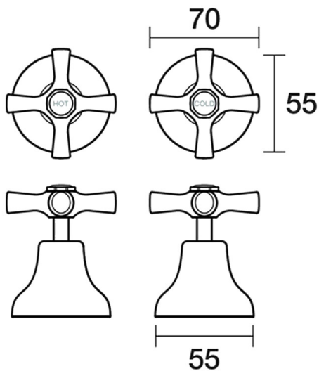
Bell Top Assemblies Hob Pair B32.083.1.03 - Chrome / White
