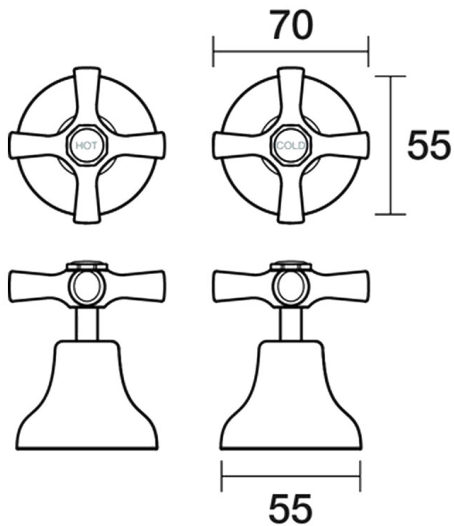
Bell Top Assemblies Hob Pair B32.083.1.12 - 23k Brushed Gold
