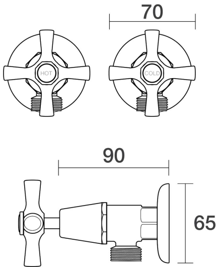
Bell Washing Machine Stops Wall Pair Ceramic Disc 091.2.04 - Chrome / Ivory
