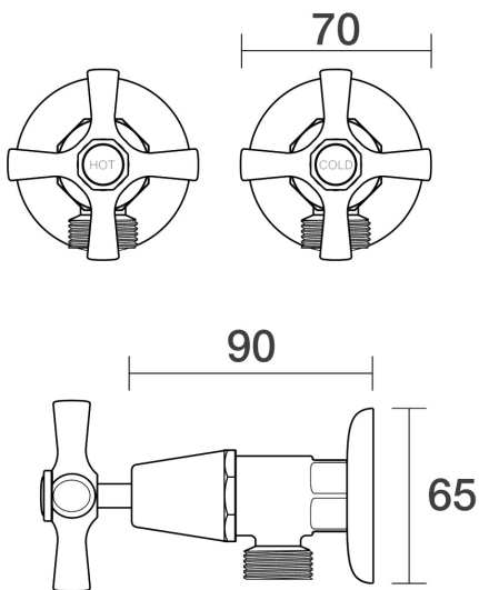
Bell Washing Machine Stops Wall Pair Ceramic Disc 091.2.17 - Gold / Victorian Green
