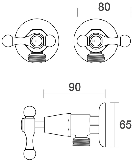
Bell Washing Machine Stops Wall Pair Lever Ceramic Disc B32.091.3.03 - Chrome / White
