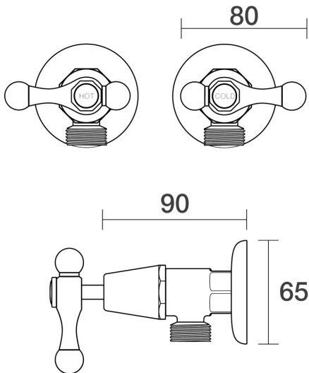
Bell Washing Machine Stops Wall Pair Lever Ceramic Disc
