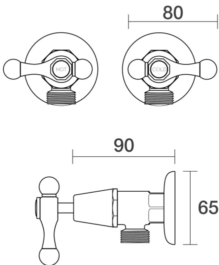
Bell Washing Machine Stops Wall Pair Lever Ceramic Disc B32.091.3.13 - Gold / White
