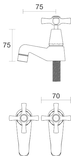
Bell Pillar Taps Pair B32.111.1.01 - Chrome
