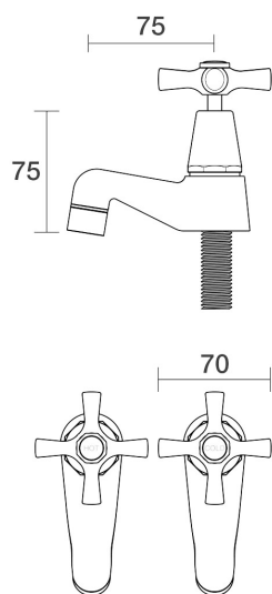
Bell Pillar Taps Pair Ceramic Disc B32.111.2.19 - 23k Brushed Brass Gold
