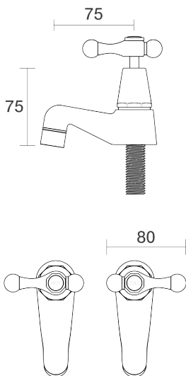
Bell Pillar Taps Pair Lever Ceramic Disc B32.111.3.01 - Chrome
