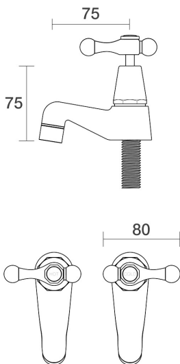
Bell Pillar Taps Pair Lever Ceramic Disc B32.111.3.10 - Chrome / Gold
