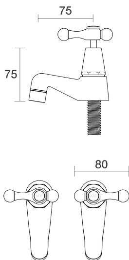
Bell Pillar Taps Pair Lever Ceramic Disc B32.111.3.14 - Gold / Ivory
