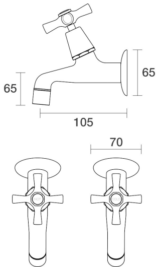
Bell Female Bibs Wall Pair Ceramic Disc B32.121.2.19 - 23k Brushed Brass Gold .19
