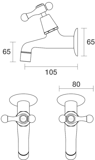
Bell Female Bibs Wall Pair Lever Ceramic Disc B32.121.3.12 - 23k Brushed Gold
