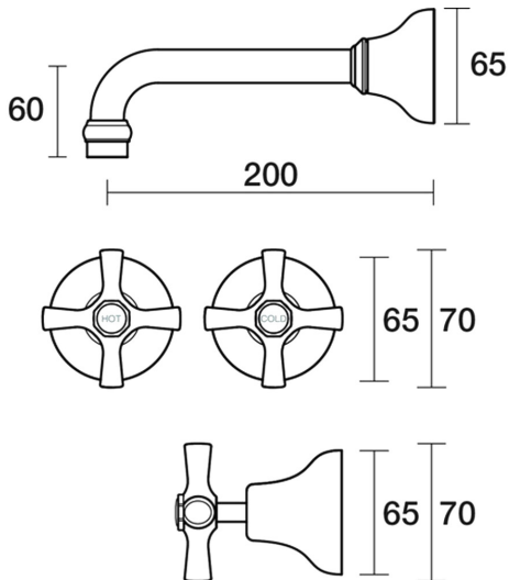
Bell Wall Basin Set 200mm Outlet Ceramic Disc B32.152.2.07 - Chrome / Victorian Green
